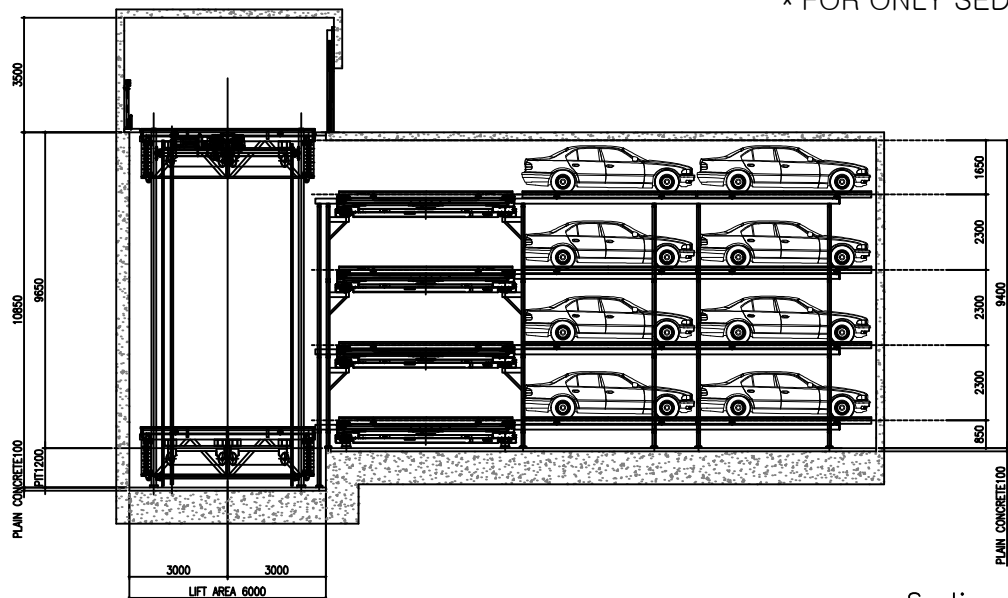
Section View
