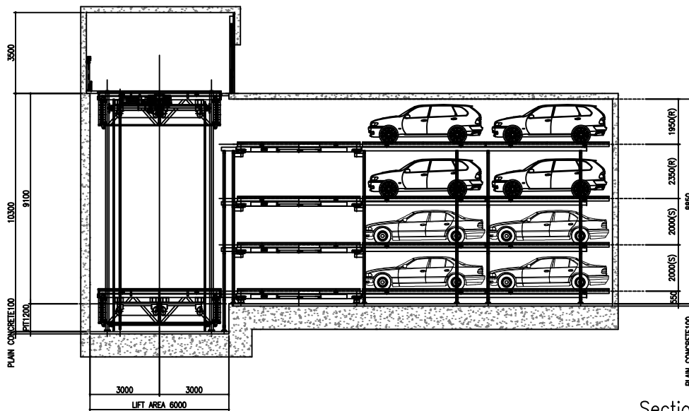
Section View
