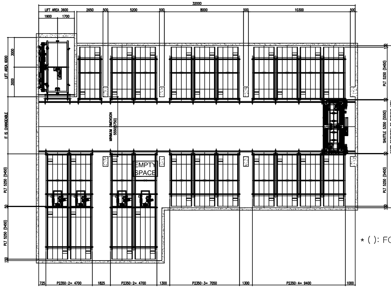
Parking Plan
