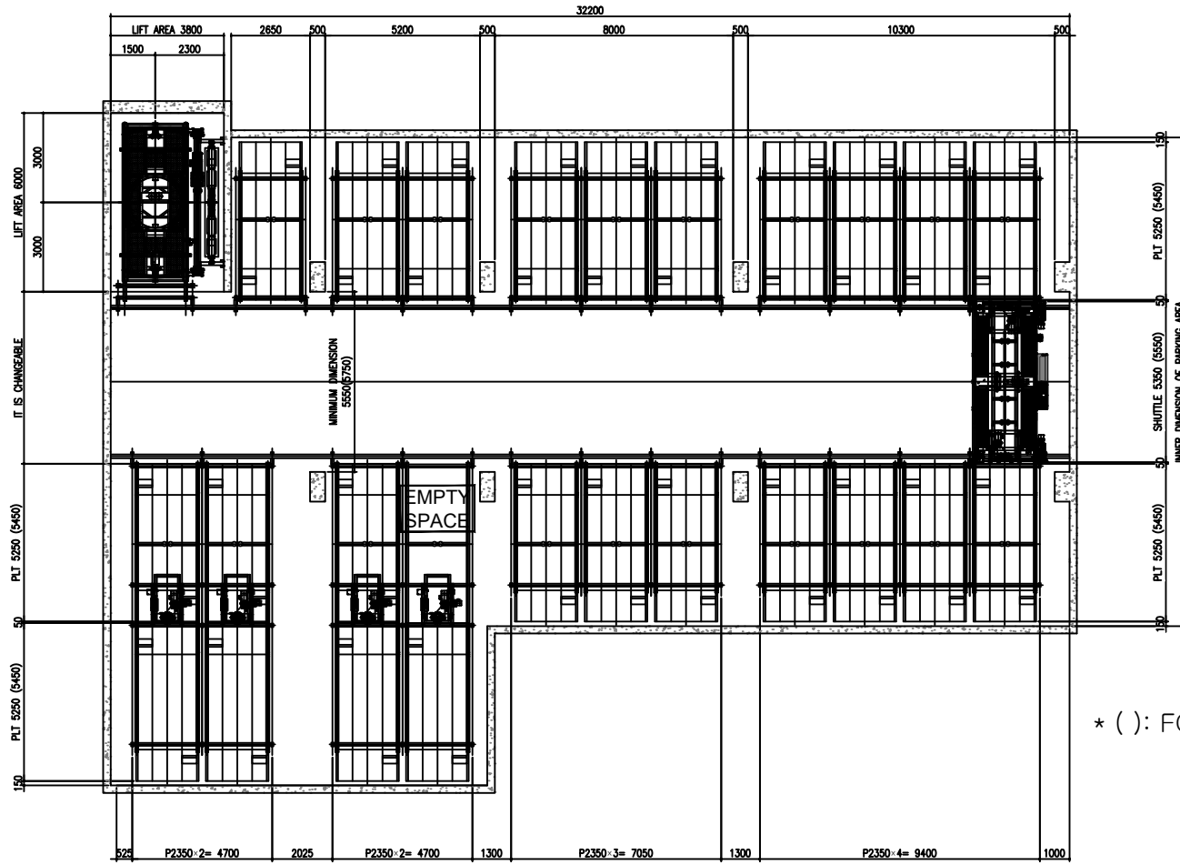
Parking Plan
