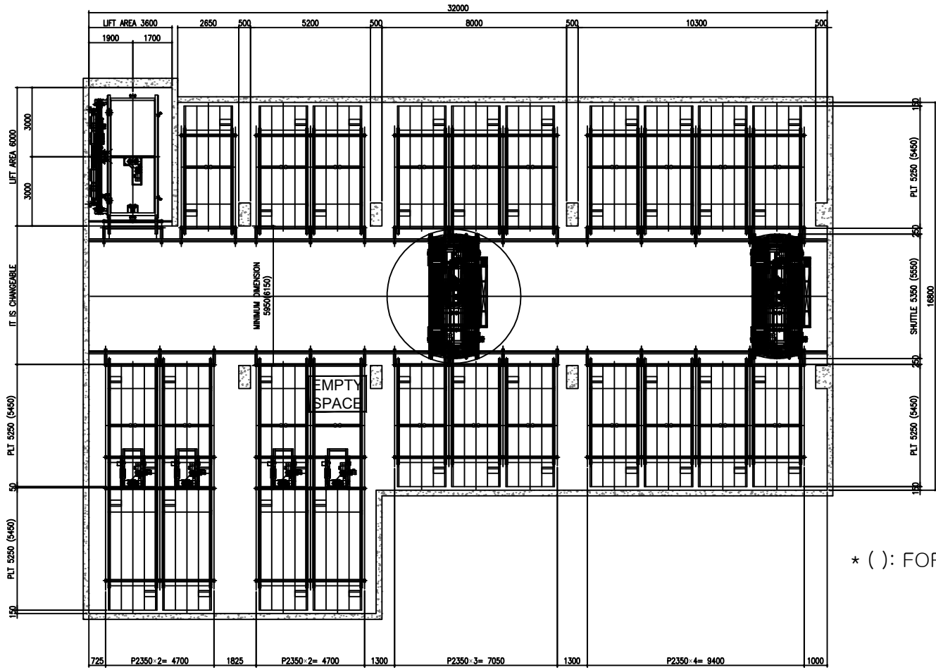
Parking Plan
