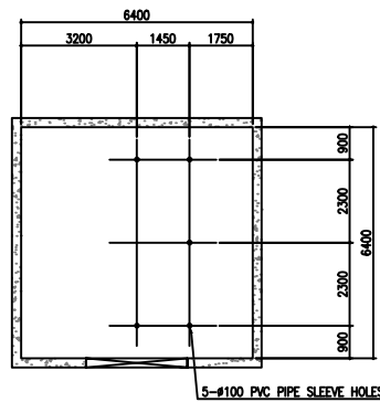
Hoisting Hook Plan
