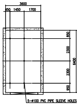
Hoisting Hook Plan
