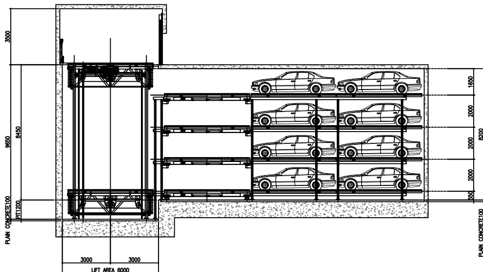
Section View
