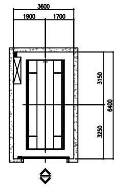
Entrance Plan
