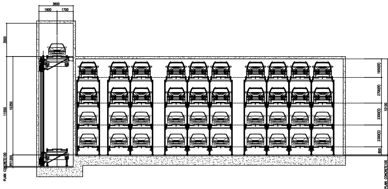
Parking Plan
