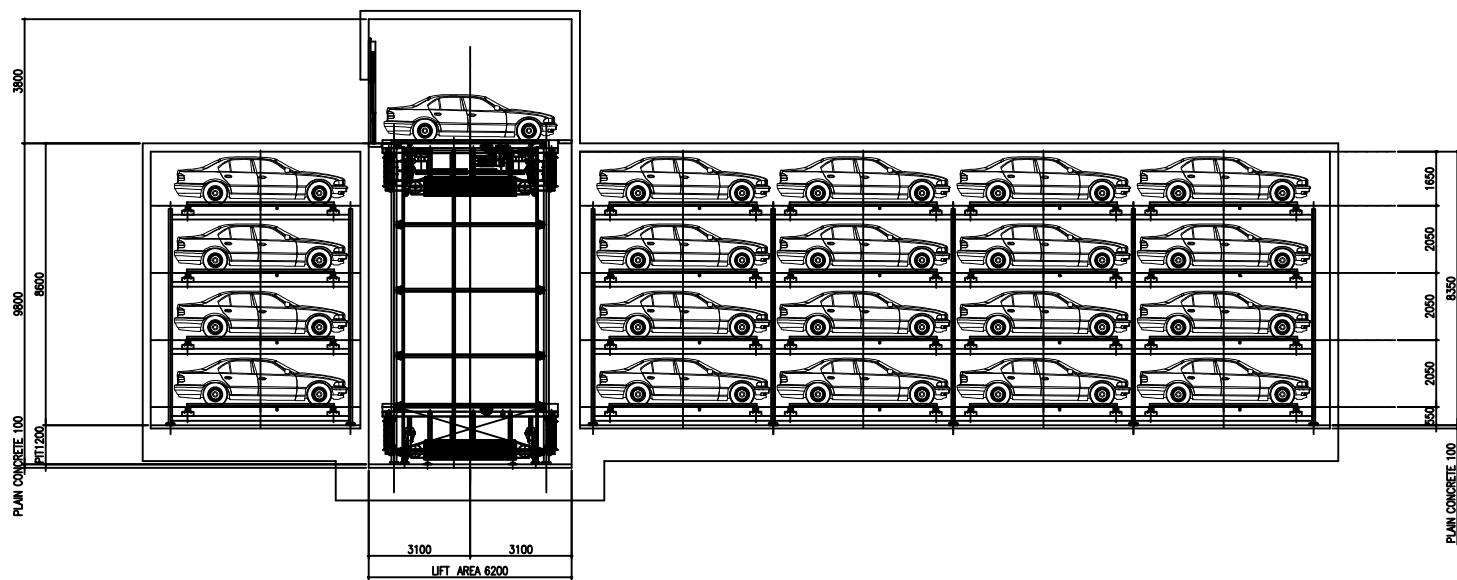
Section View
