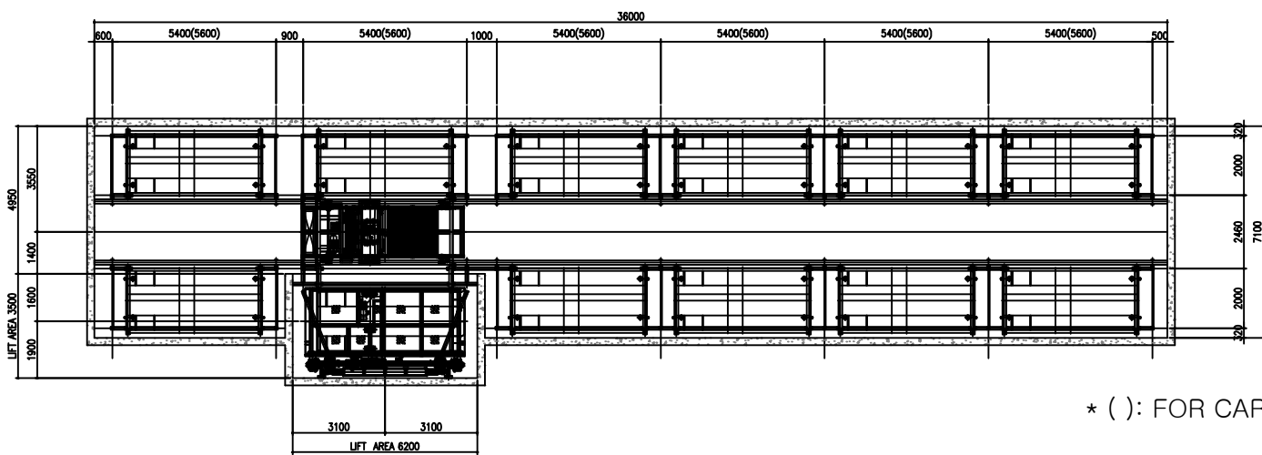
Parking Plan
