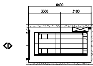
Entrance Plan
