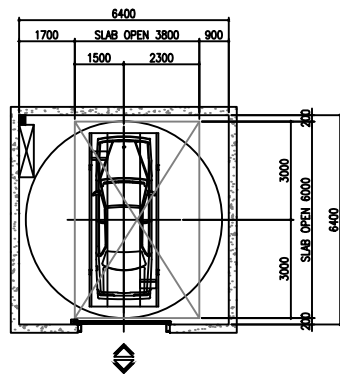
Entrance Plan
